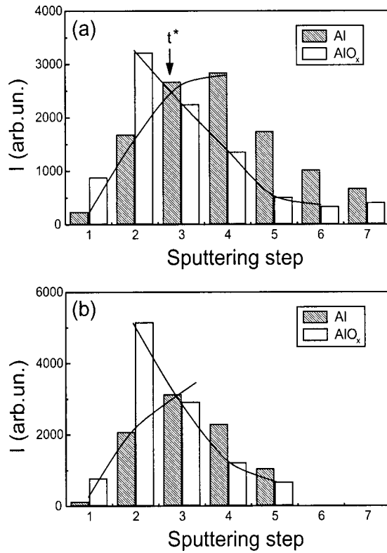
FIG. 4. Depth profile showing the fitted intensities of the Al and \text{AlO}_x contributions to the (\text{Al} + \text{AlO}_x) 2p spectra, for samples (a) W_{\text{AIR}} (t_{\text{Al}} = 8 \text{ nm}) and (b) W_{\text{AIR}} (t_{\text{Al}} = 4 \text{ nm}) . t^* indicates the sputtering time for which I(\text{AlO}_x) = I(\text{Al}) . Solids lines—intensity as a function of sputtering step—are a guide for the eyes.
