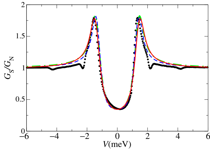
Figure 1. Normalized tunnelling conductance of junction 1 measured at T = 1.52 K. Black circles indicate experimental data; dashed-dotted green lines are fits to model I, dashed blue, fits to model II, and solid red, fits to model III.
