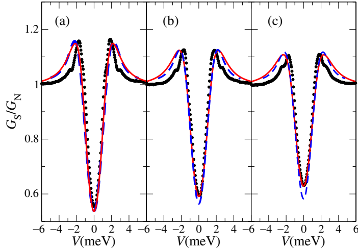
Figure 3. Normalized tunnelling conductance of junction 3 measured at T = 4.53 K (a), 5.0 K (b) and 5.39 K (c), together with a fit to models II (dashed blue) and III (solid red).
