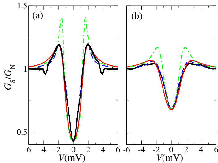
Figure 2. Normalized tunnelling conductance of junction 2 measured at T = 1.5 K (a) and 3.945 K (b), together with a fit to models I (dash-dotted green), II (dashed blue) and III (solid red).
