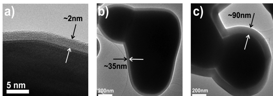
Figure 3. TEM images showing the Y@Al core–shell structure. The images display good distribution and homogeneity of the Al 2 O 3 shell (gray coating) around the core grains. The arrows at the edges of the Y@Al nanocomposite indicate the thickness of the Al 2 O 3 shell of about 2 nm (a), 35 nm (b), and 90 nm (c), corresponding to 50, 500, and 1000 ALD cycles, respectively.
